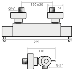
ST10010CP Acura safe touch thermostatic bar shower
