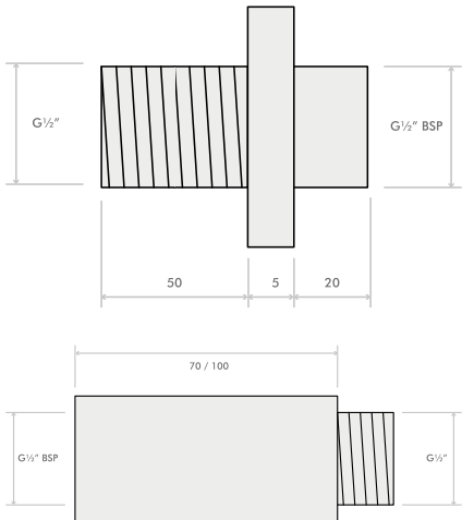
ID0063 Wall extension 1/2" M x 1/2" BSP 100mm
